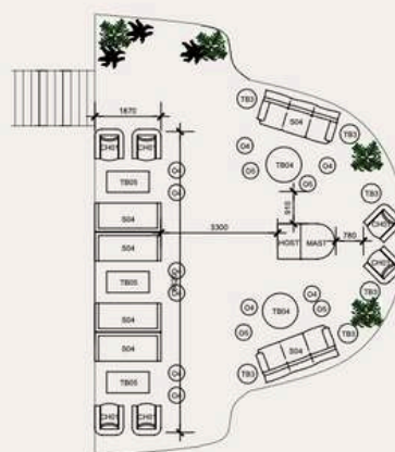
TOP DECK
