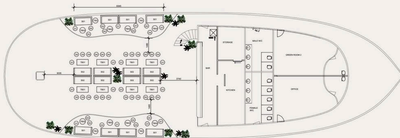
MAIN DECK
